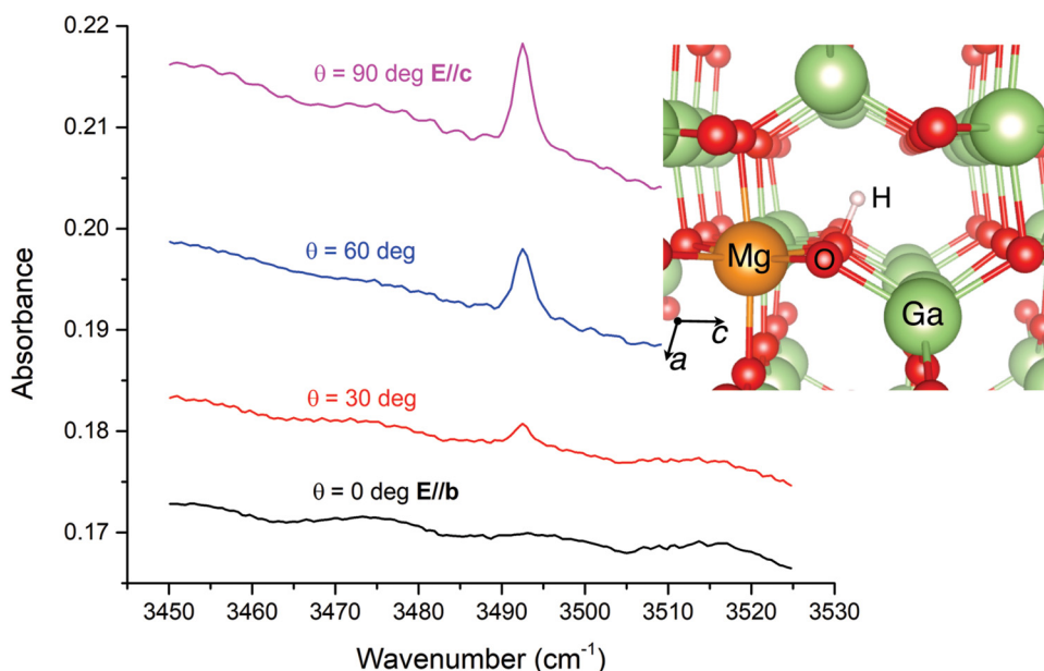
FIG. 12. Polarized IR transmission spectra of the MgH complex. The structure of the complex obtained from first-principles calculations is shown in the inset. Reprinted with permission from Ritter et al. , Appl. Phys. Lett. 113 , 052101 (2018). Copyright 2018 AIP Publishing. 79
