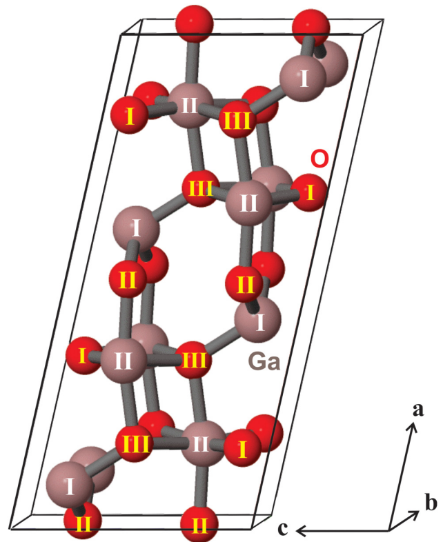
FIG. 2. Crystal structure of monoclinic \beta -Ga 2 O 3 . Some of the bonds, which extend to atoms in neighboring unit cells, are not shown. Figure made using a #3Dview from Ahman et al. , Acta Cryst. C 52, 1336 (1996). Copyright 1996 @IUCr.
