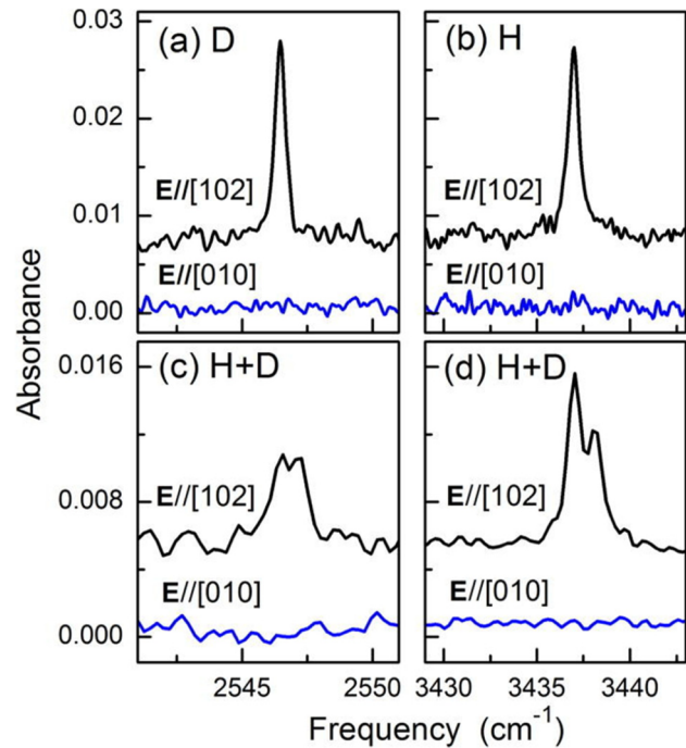
FIG. 10. IR transmission spectra of V_{\text{Ga}}2\text{H} complexes. Samples with a mixture of H and D show new peaks that correspond to V_{\text{Ga}}\text{HD} centers. IR light polarization along [010] is perpendicular to O–H bonds and is not absorbed. Spectra reprinted with permission from Weiser et al. , Appl. Phys. Lett. 112 , 232104 (2018). Copyright 2018 AIP Publishing. 64
